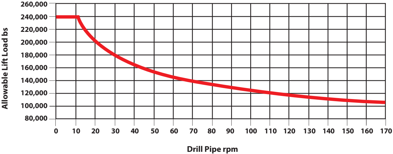
Performance Data 10.12 cu in Pump, 5,000 psi max
