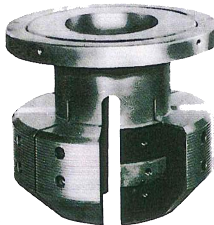
Slip Carrier for 11-3/4" to 18-3/4" O.D. Spear for 18-5/8" to 30" Casing
